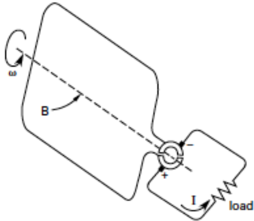
Figure 11: Commutator Action
