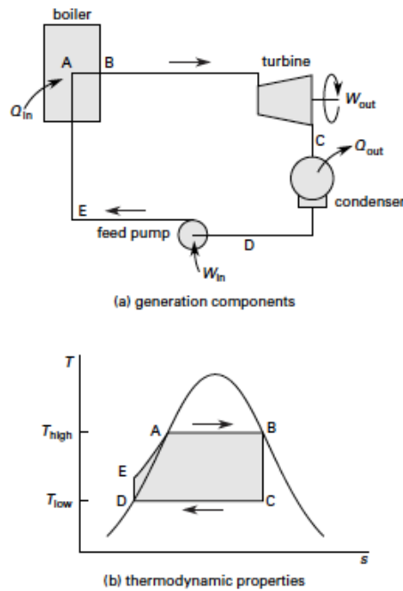
Figure 1: Basic Rankine Cycle
