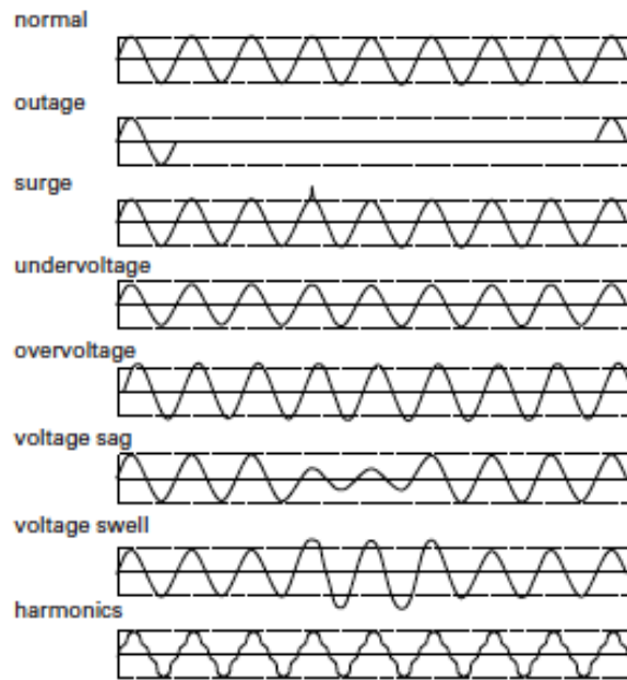
Figure 15: Power Disturbances
