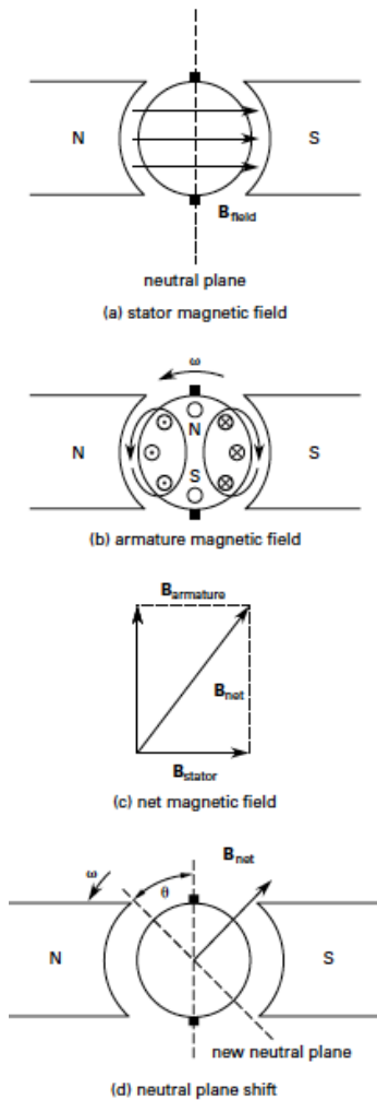
Figure 13: DC Generator Armature Flux
