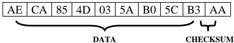
Figure 7 - Packet of Data Containing 8-bit Checksum
