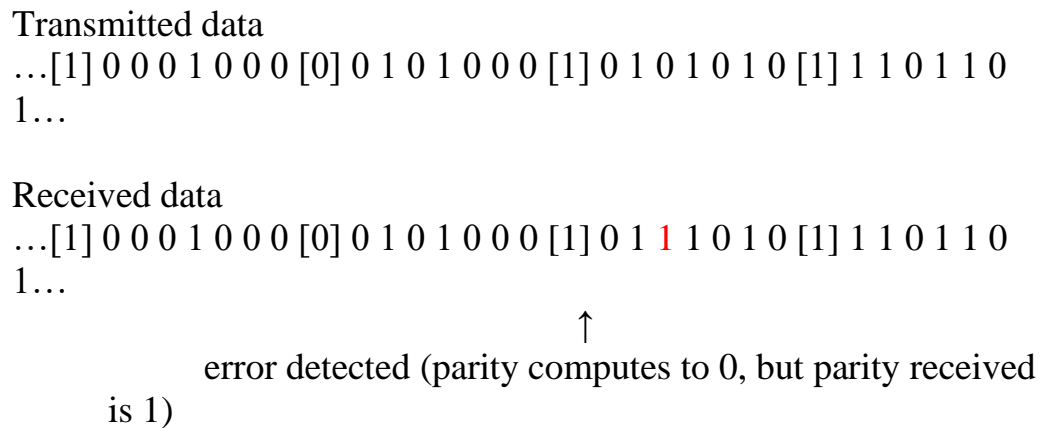
Figure 3 - Example of Data Transmission and Error Detection
